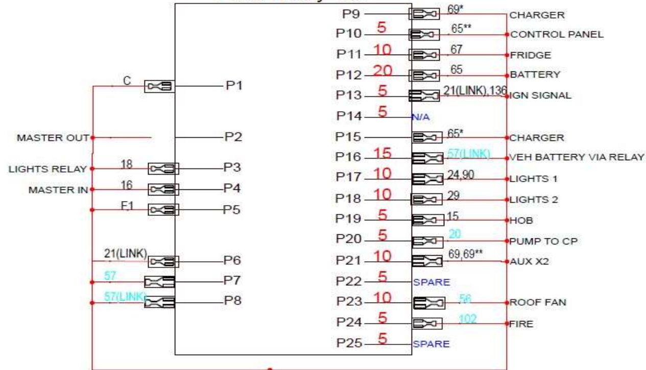
Fuse Relay 184
