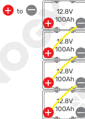
Series Connection 48V(51.2V) 100Ah
