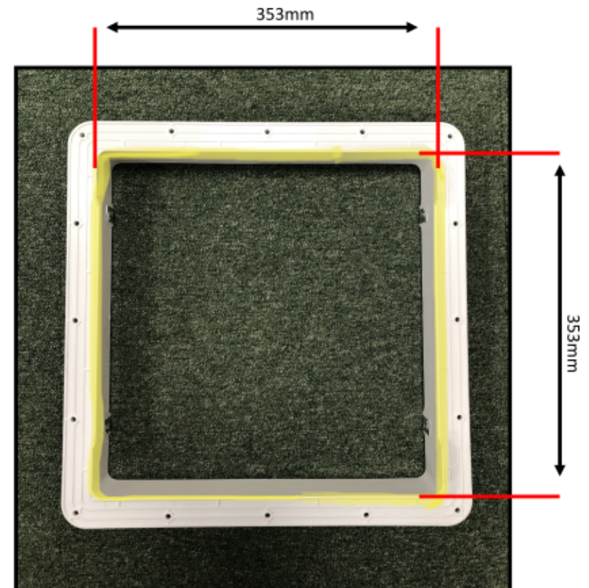
KI models = 35 x 35cm roof flange
